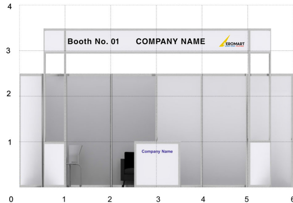
FRONT ELEVATION (NTS) Booth Size: 6m (L) x 4m (W) x 3.5m (H)
